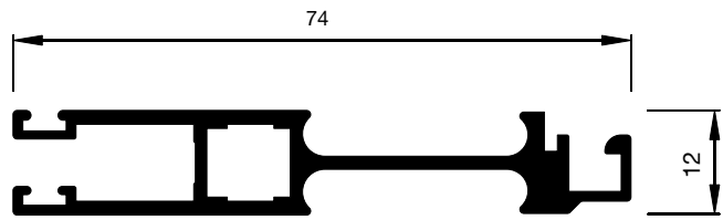
A1.3011 1274ST
