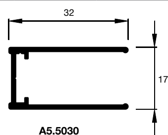
A5.5030 Wandprofil
